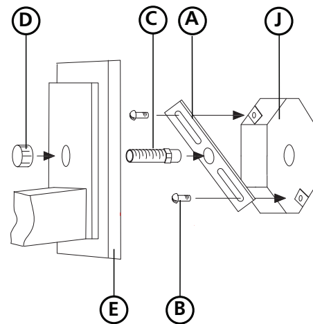
Drawing 2 - Assembly
